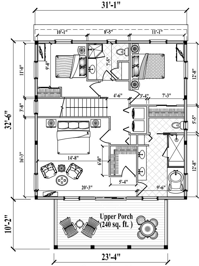
Upper Floor Plan (1,015 sq. ft. or 94.3 m 2 )
