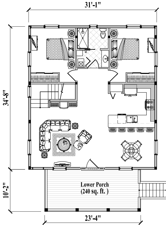
Lower Floor Plan (1,085 sq. ft. or 100.7 m 2 )
