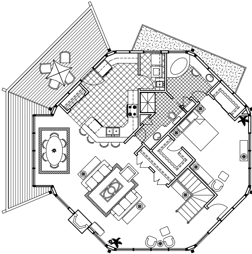
Upper Floor Plan (1,305 sq. ft.)
