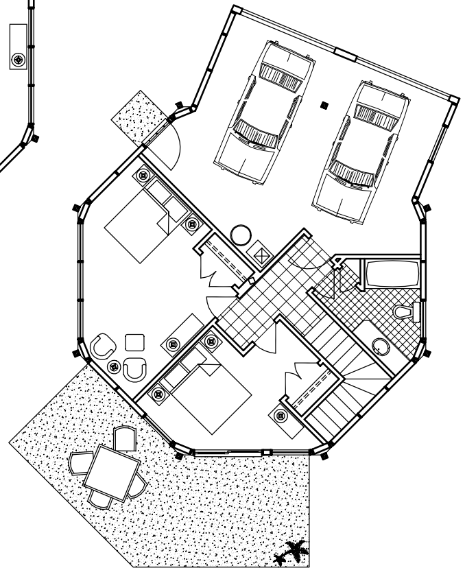
Lower Floor Plan (950 sq. ft.)
