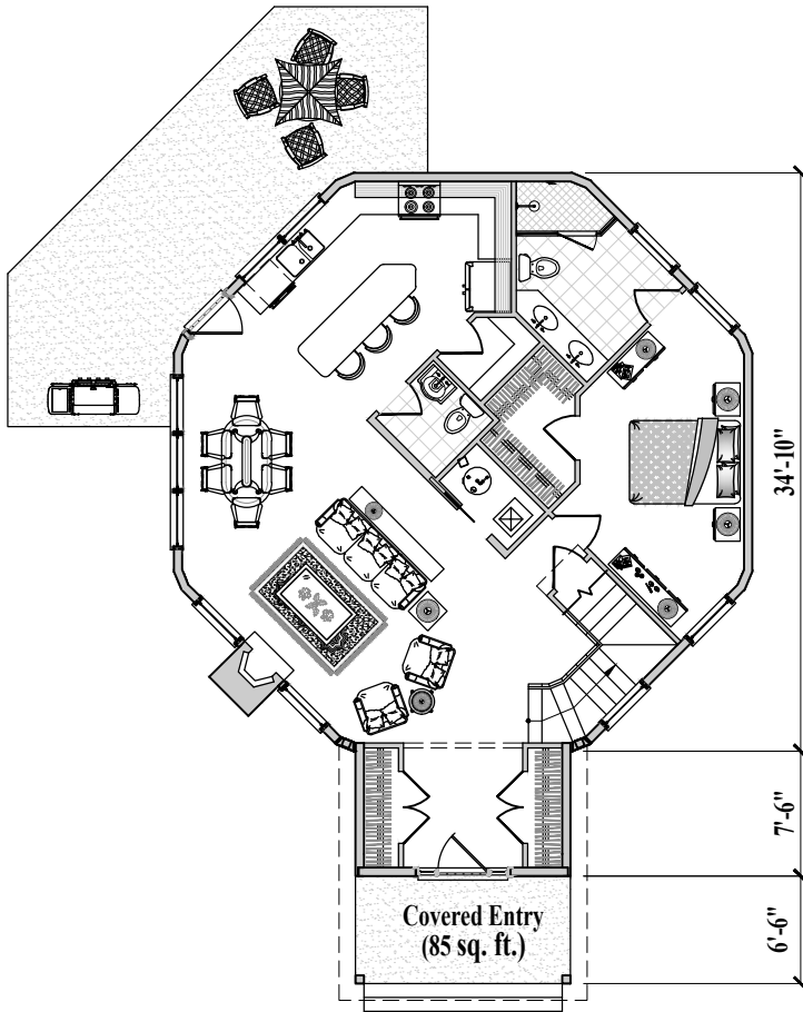
Lower Level Floor Plan (1,105 sq. ft. or 100m 2 )
