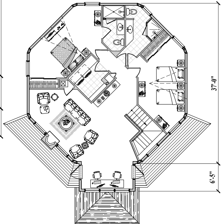
Upper Level Floor Plan (1,225 sq. ft. or 115 m 2 )
