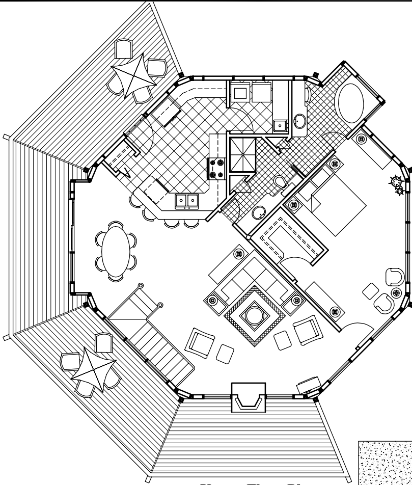
Upper Floor Plan (1,175 sq. ft.)
