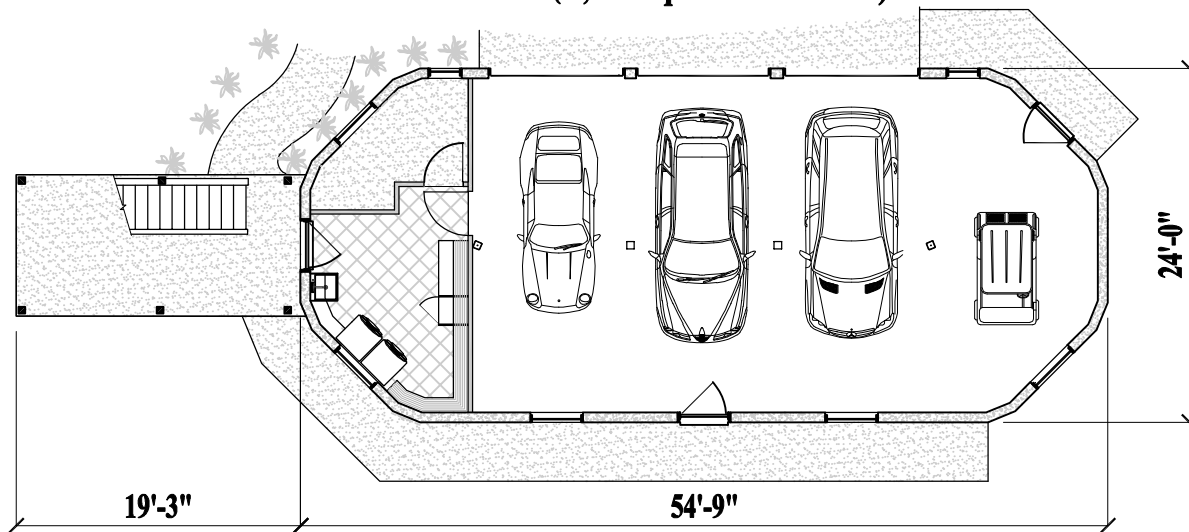
Lower Floor Plan (Conditioned 230 sq. ft. or 21.4 m 2 ) Garage 980 sq. ft. or 91 m 2 )
