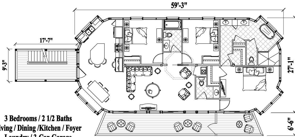
Upper Floor Plan (1,510 sq. ft. or 140.3 m 2 )
