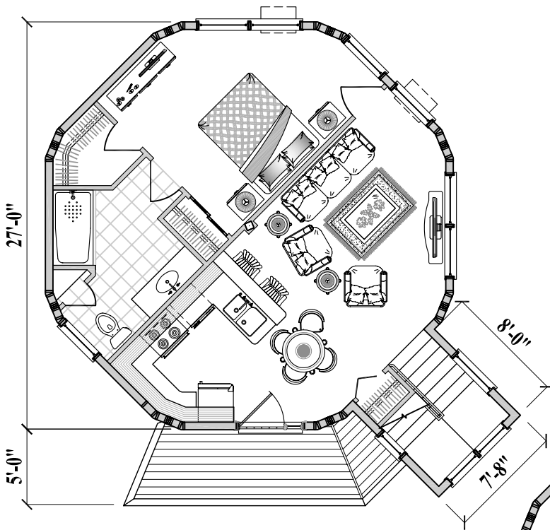
Upper Floor Plan (665 sq. ft. or 61.8 m 2 )
