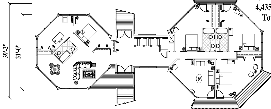
First Floor Plan (Total 2,415 sq. ft. or 224 m 2 )
