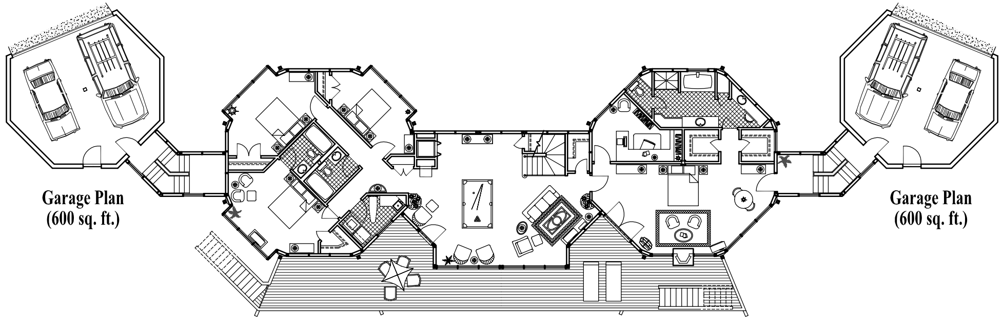
Lower Floor Plan (2,530 sq. ft.)
