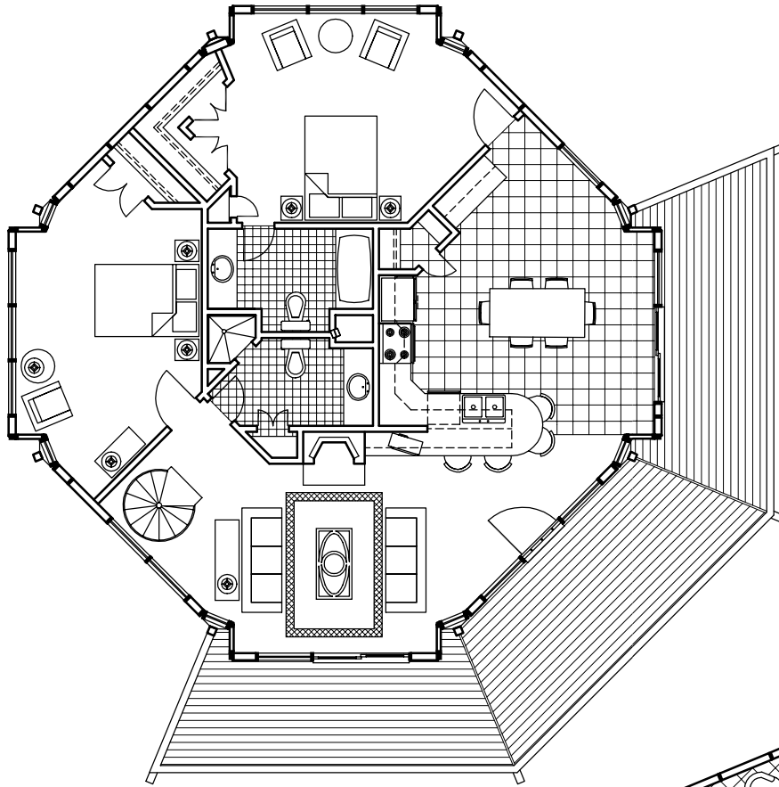
Upper Floor Plan (1,225 sq. ft.)
