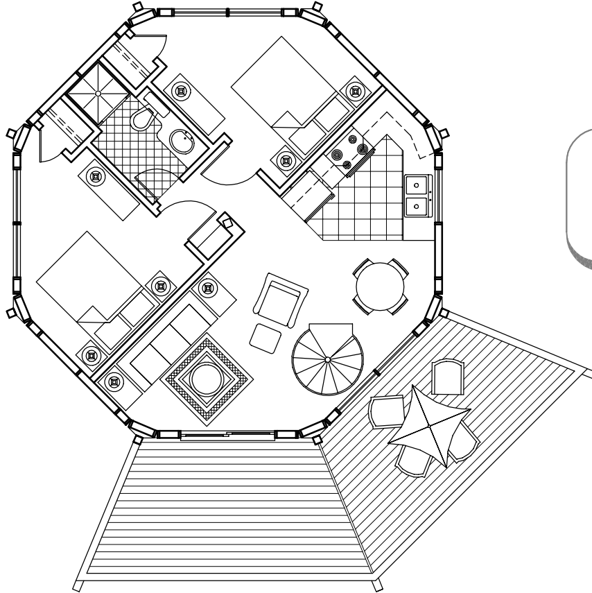
Upper Floor Plan (600 sq. ft.)
