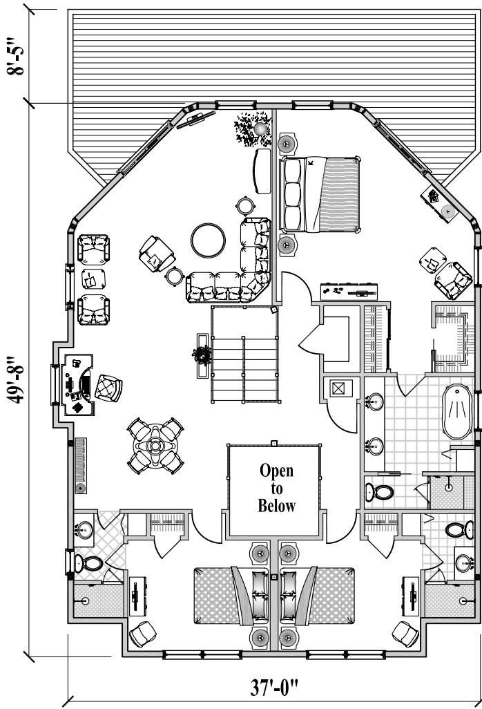
Upper Floor Plan (1,700 sq. ft. or 158 m 2 )
