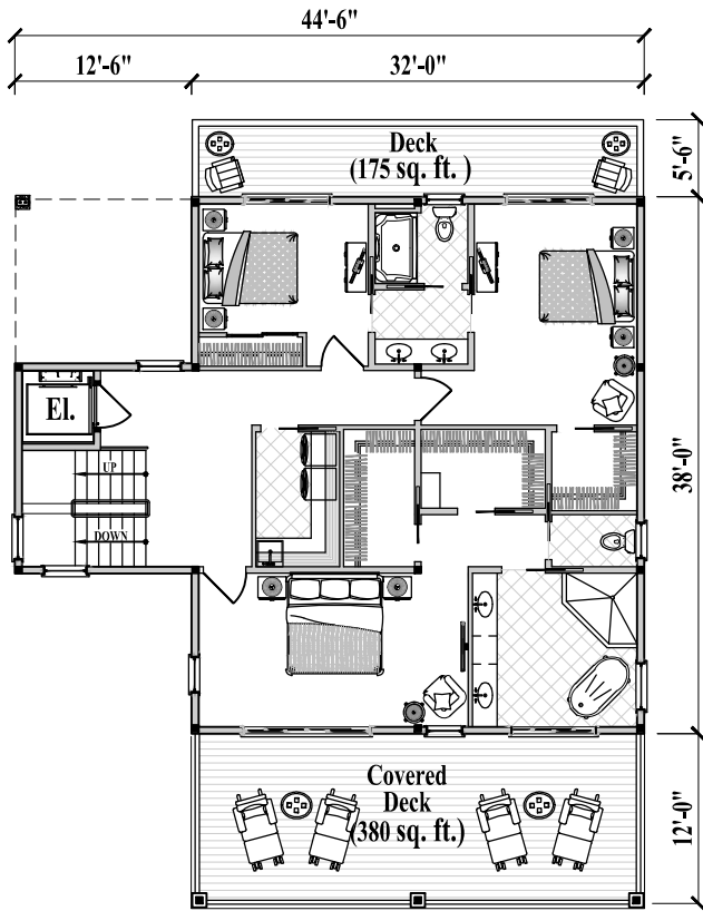
Lower Floor Plan (1,400 sq. ft. or 130 m 2 )
