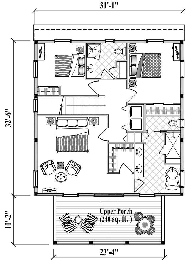
5 Bedrooms / 3 Baths Living / Dining / Kitchen Upper Floor Plan (1,015 sq. ft. or 94.3 m 2 ) (Total 2,220 sq. ft. or 206.1 m 2 )
