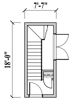
Lower Floor Plan (140 sq. ft. or 13 m 2 )
