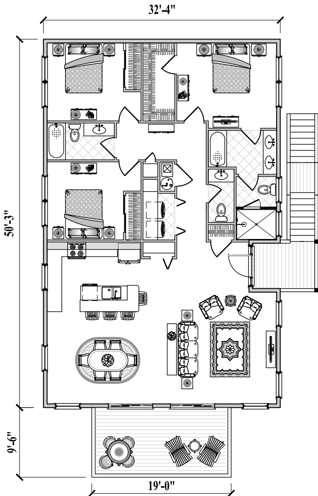
Floor Plan (1,600 sq. ft. or 148 m 2 )
