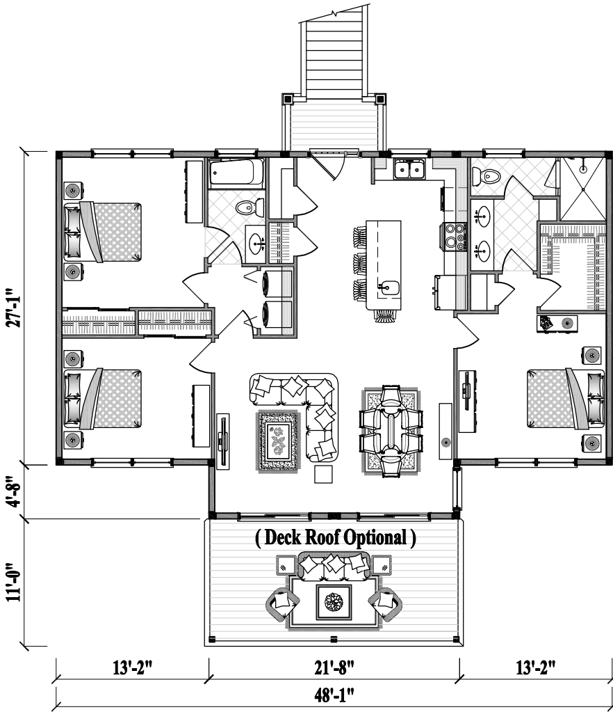
Floor Plan (1,400 sq. ft. or 130 m 2 )
