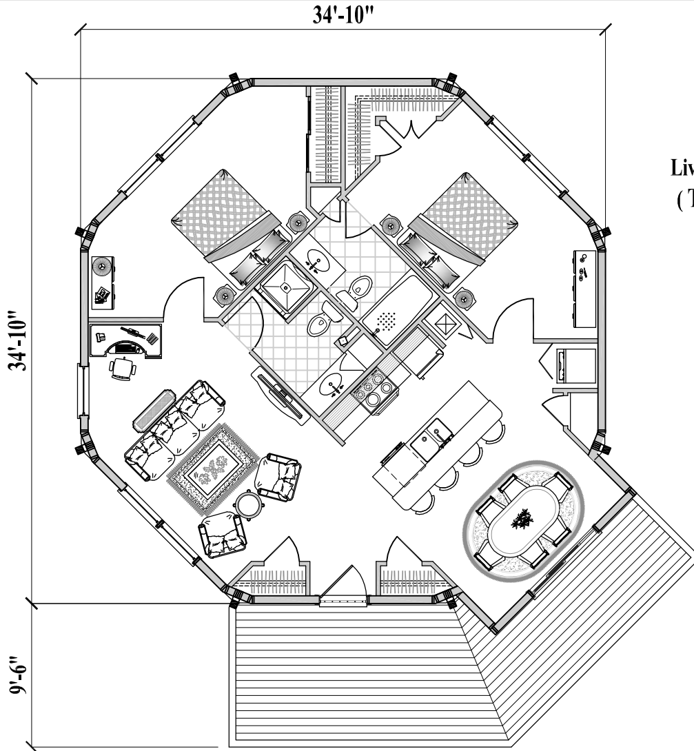
Floor Plan (Total 1,050 sq. ft. or 98 m 2 )
