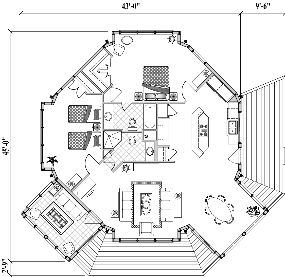
Floor Plan ( Total 1,460 sq. ft. or 135 m 2 )
