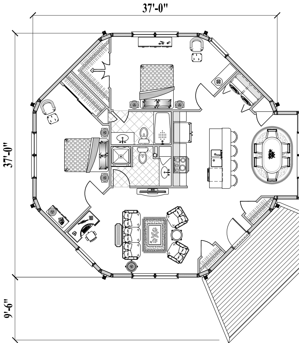
Floor Plan (Total 1,175 sq. ft. or 109 m 2 )
