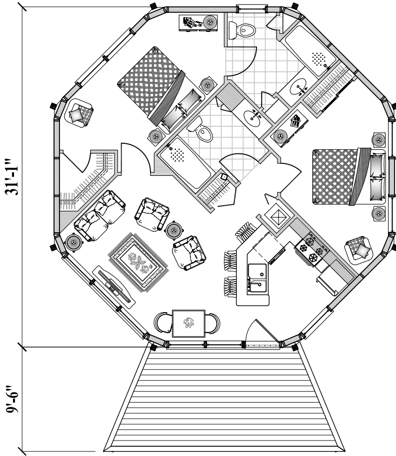
Floor Plan (Total 800 sq. ft. or 74 m 2 )
