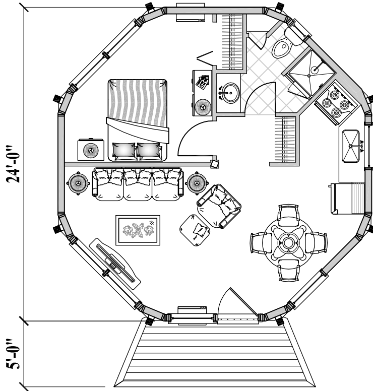
Floor Plan (Total 475 sq. ft. or 44 m 2 )
