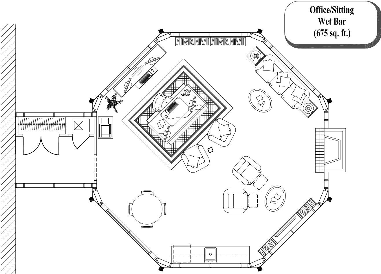
Floor Plan (675 sq. ft.)
