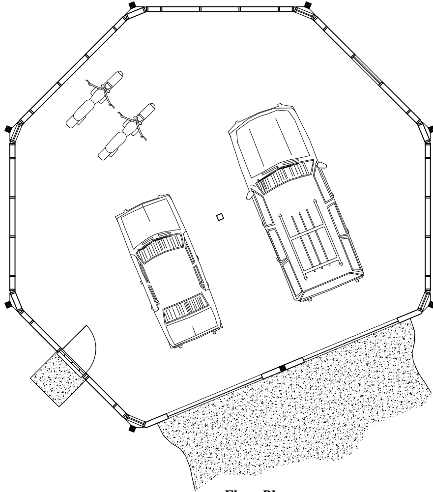
Floor Plan (1,125 sq. ft.)
