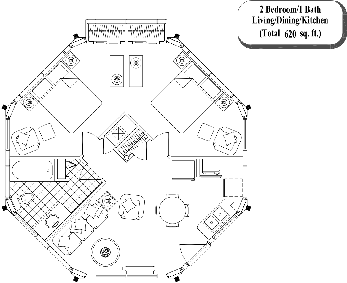
Floor Plan (620 sq. ft.)
