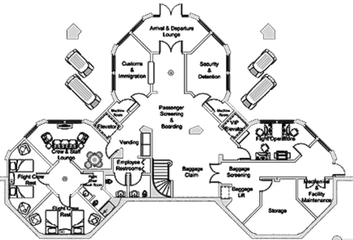
Arrival - Departure Level Plan
