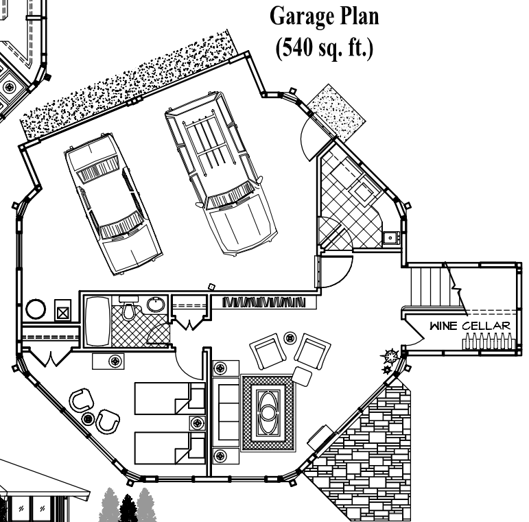
Lower Floor Plan (630 sq. ft.)
