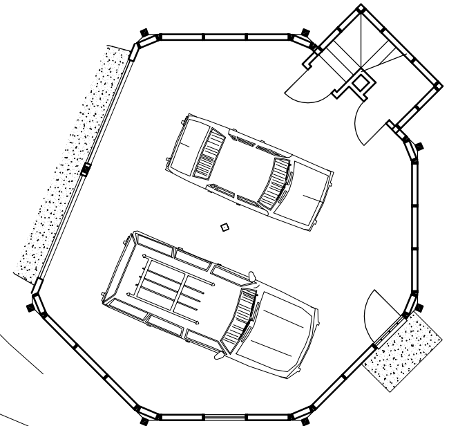
Garage Plan (850 sq. ft.)
