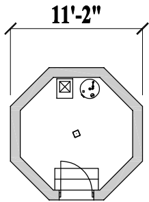
Pedestal Plan (Total 100 sq. ft. or 9 m 2 )
