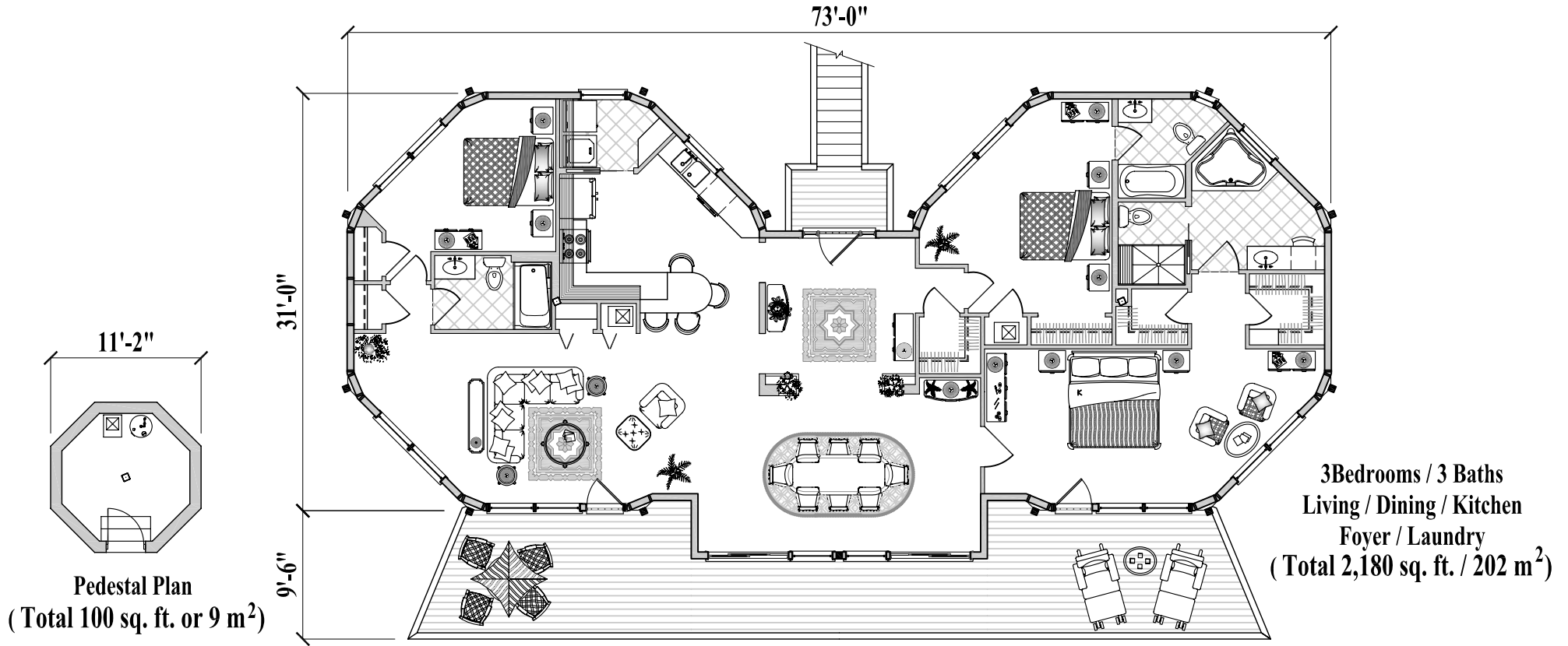
Floor Plan (1,980 sq. ft. or 184 m 2 )
