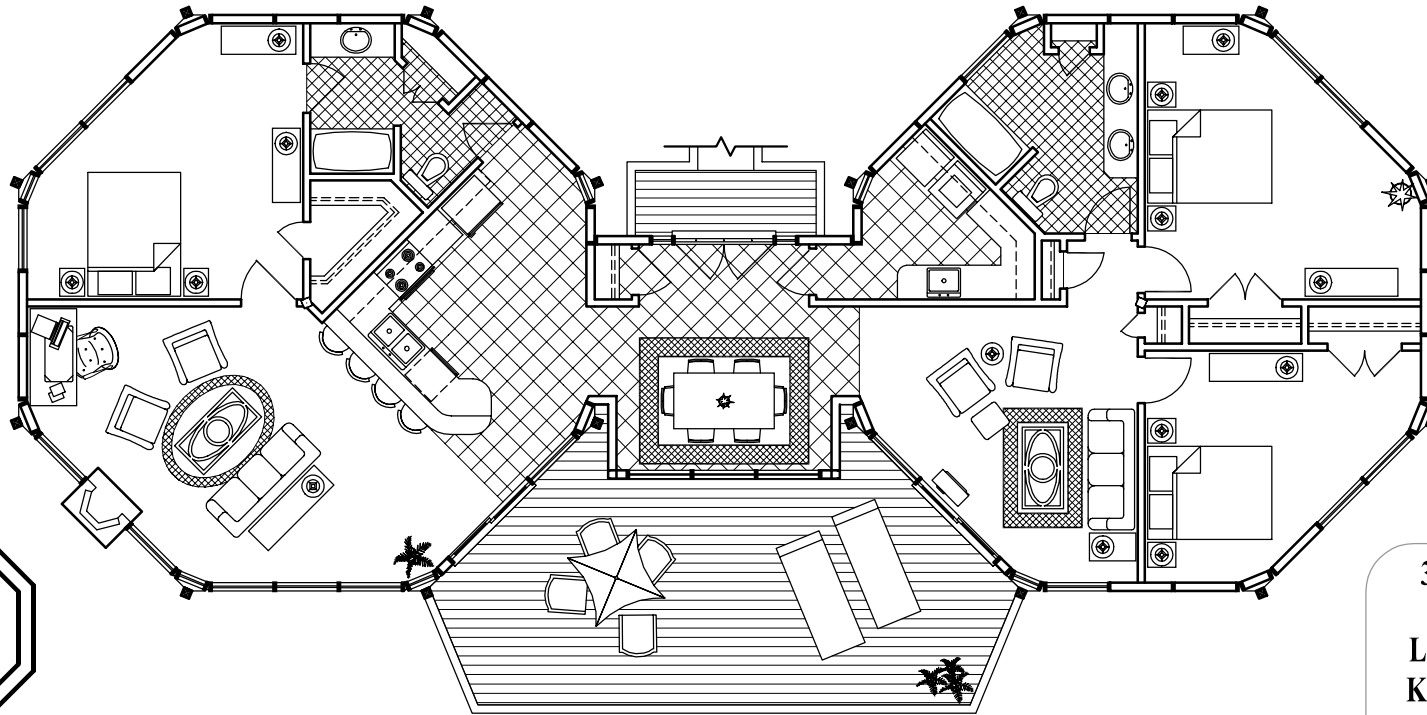
Floor Plan (1,825 sq. ft.)
