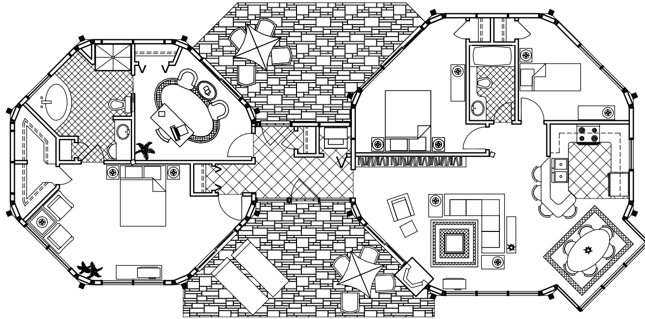
Floor Plan (1,600 sq. ft.)
