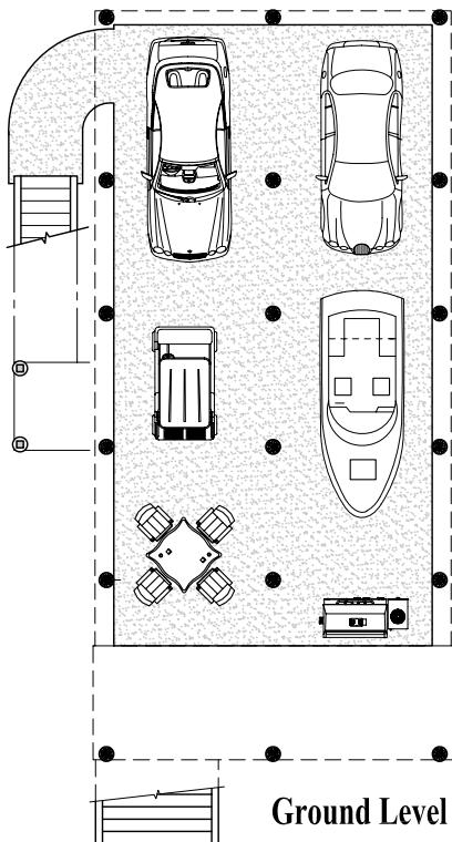
Lower Floor Plan (1,030 sq. ft. or 95.7 m 2 )
