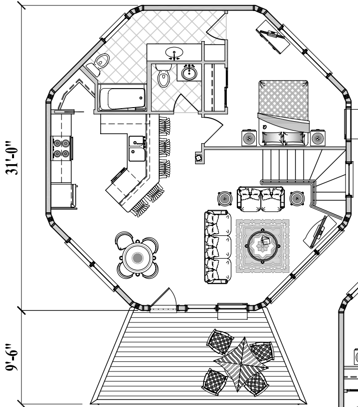
Upper Floor Plan (800 sq. ft. or 74.3 m 2 )
