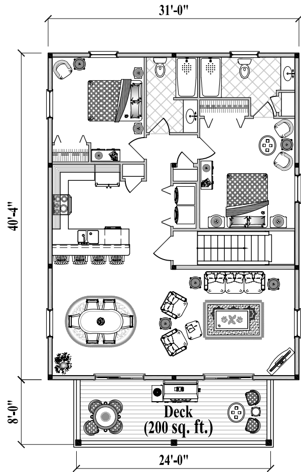
Floor Plan (1,250 sq. ft. or 116 m 2 )
