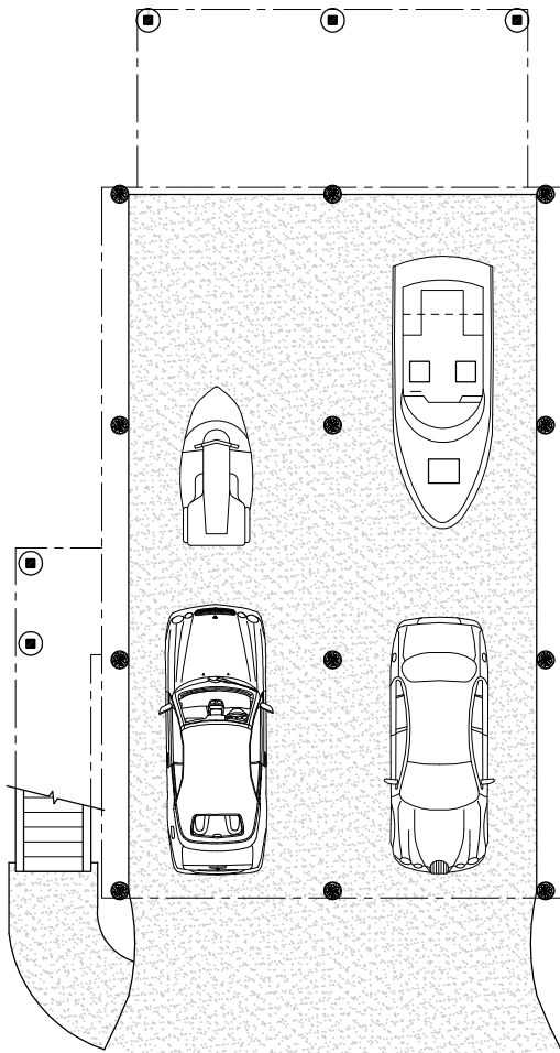
Ground level (Parking Area)
