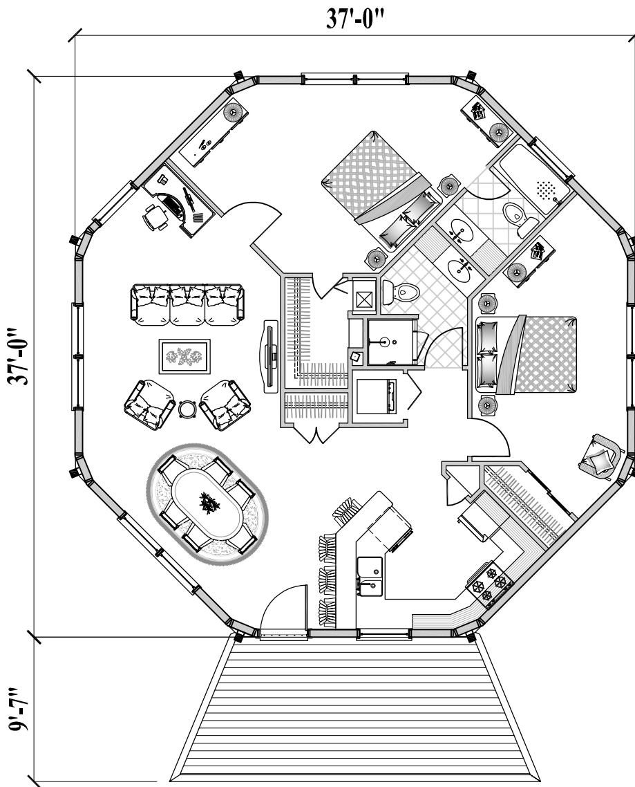
Floor Plan (Total 1,125 sq. ft. or 105 m 2 )
